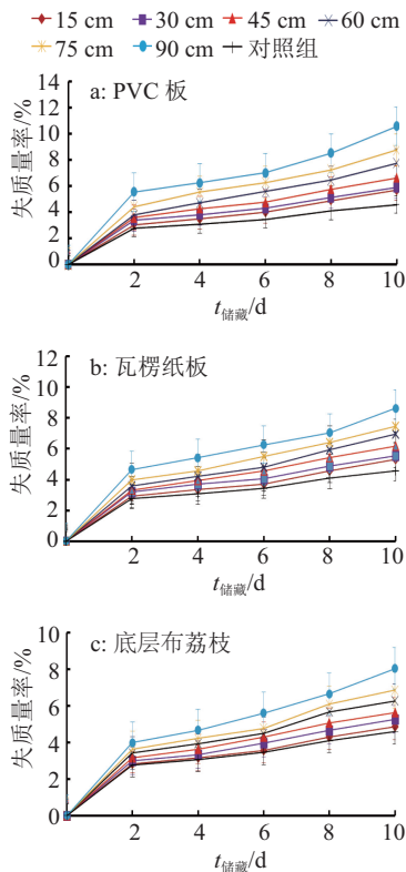
图 5 储藏时间对荔枝失质量率的影响 Fig. 5 Effect of storage time on weight loss rate of litchi
